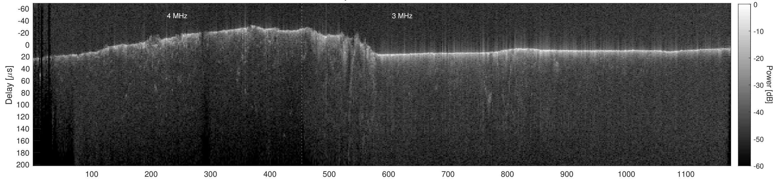
Orbit 16552, Cluttergram
