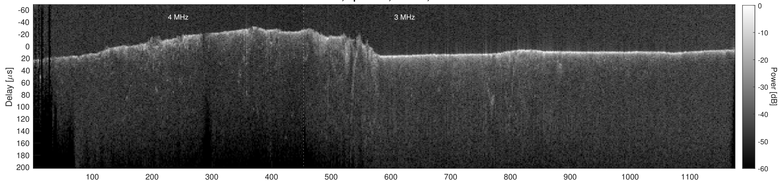
Orbit 16552, Cluttergram
