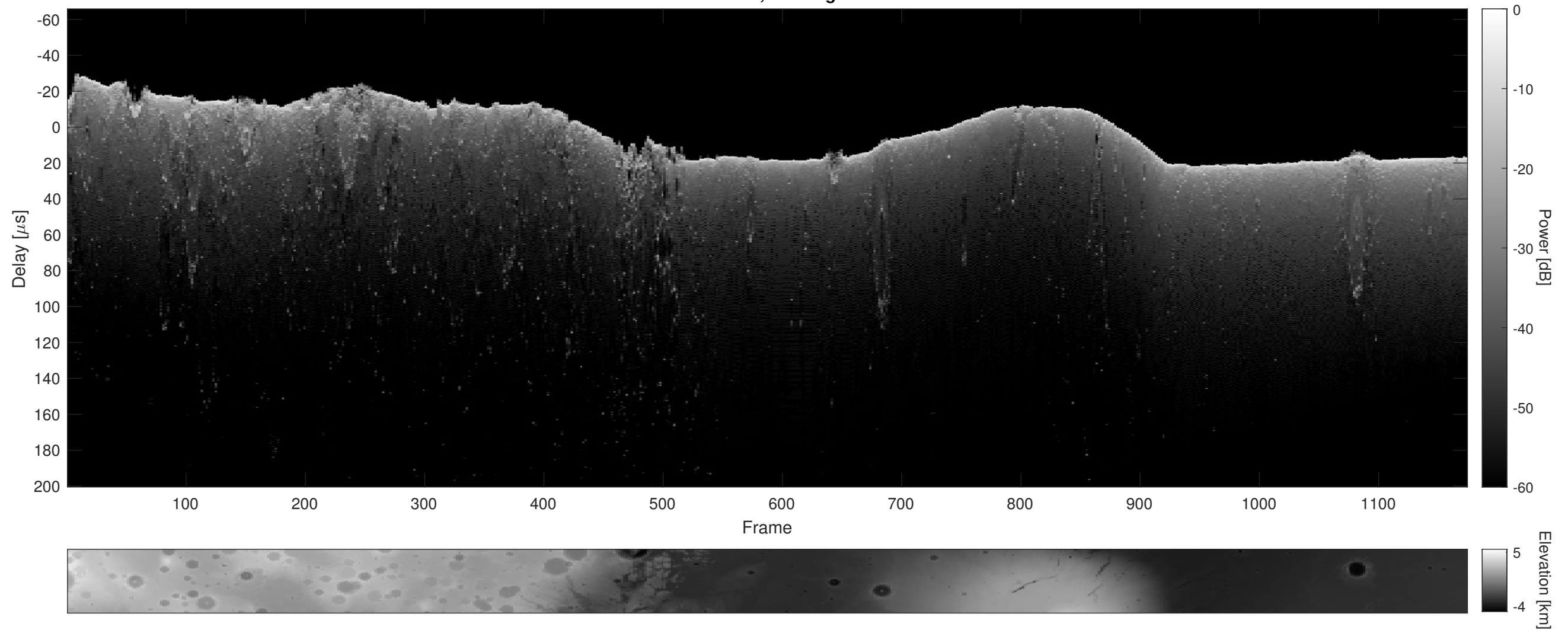
Orbit 16555, Cluttergram
