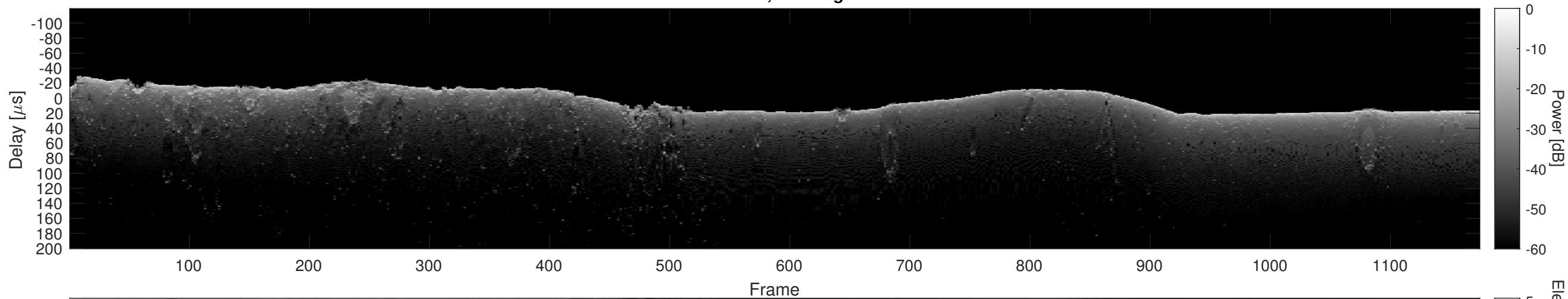
Orbit 16555, Cluttergram
