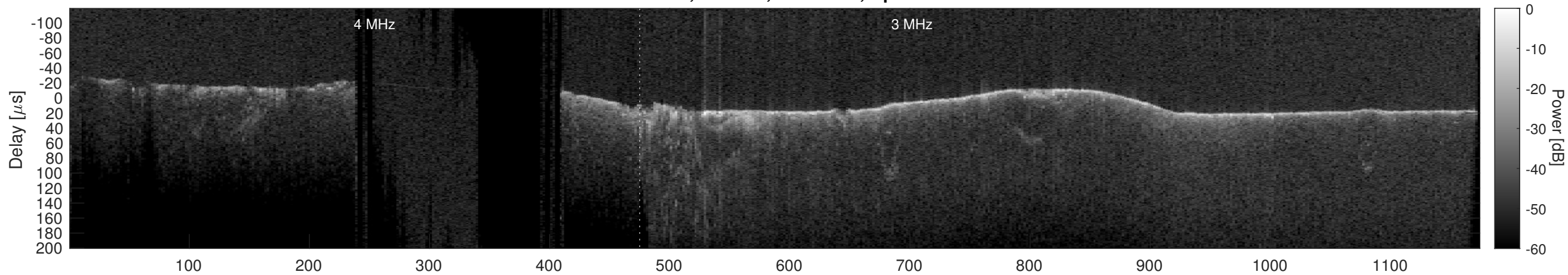
Orbit 16555, Cluttergram
