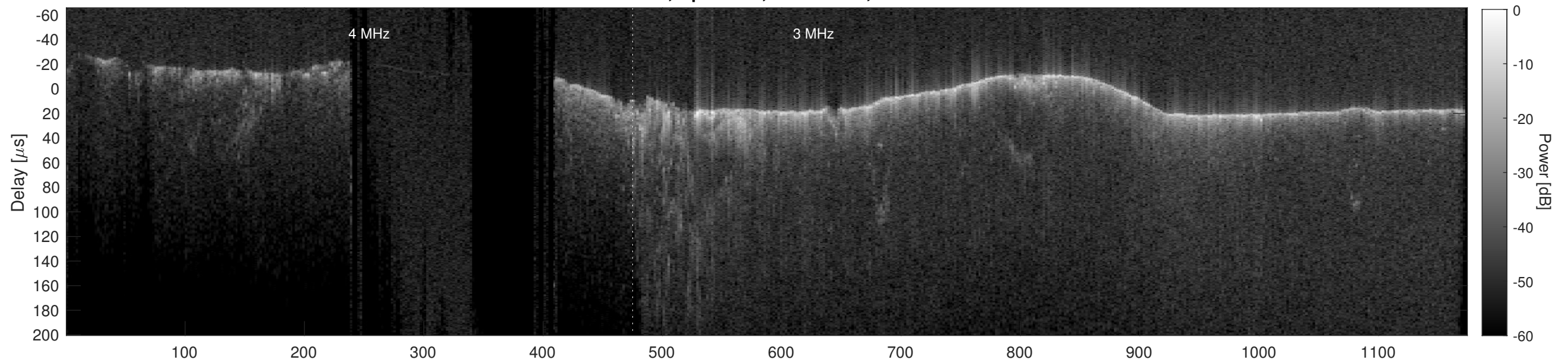
Orbit 16555, Cluttergram
