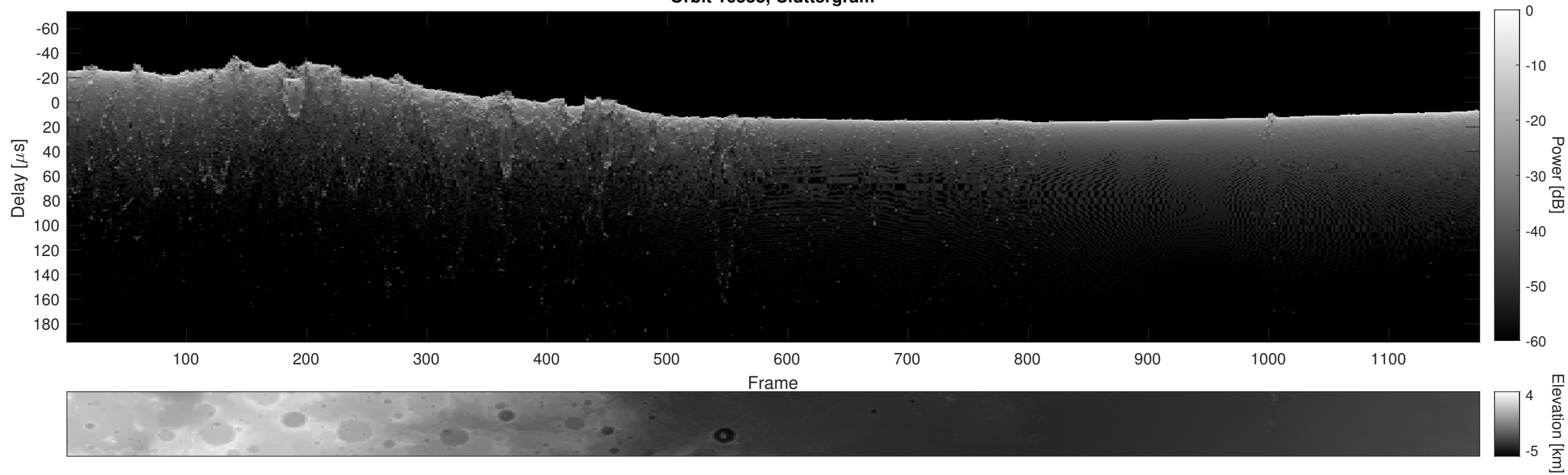
Orbit 16558, Cluttergram
