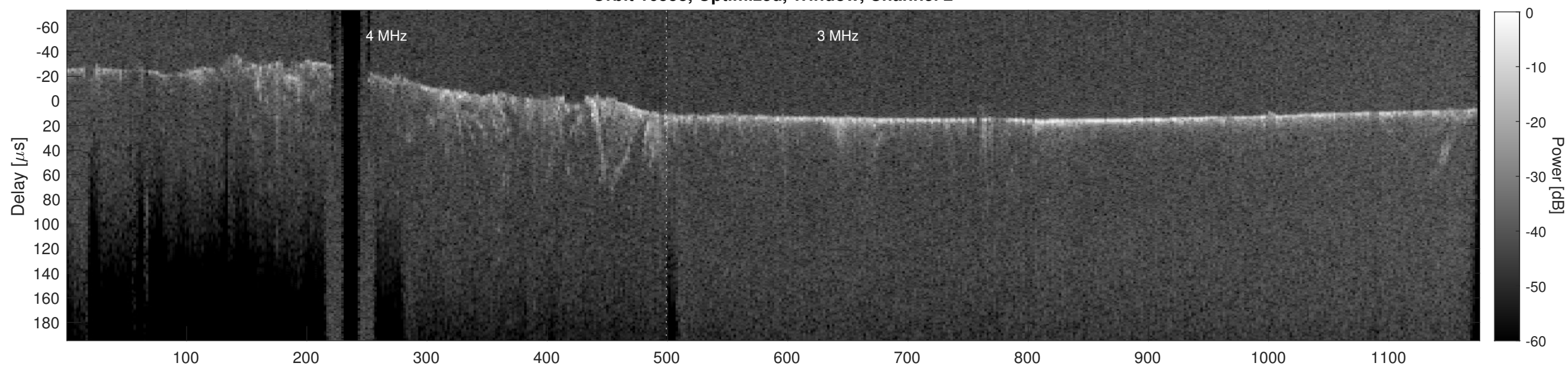
Orbit 16558, Cluttergram
