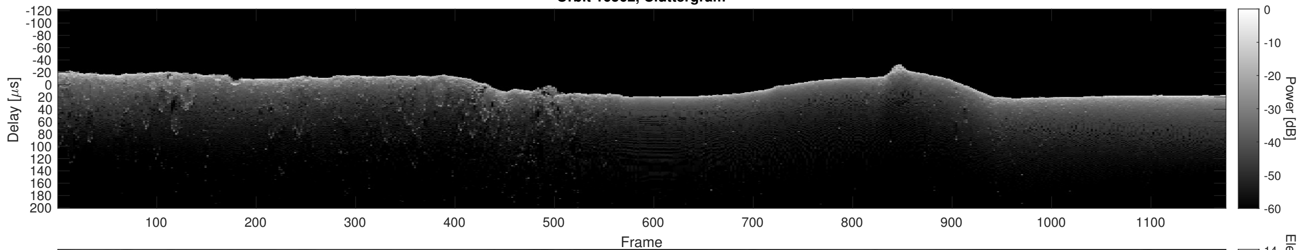
Orbit 16562, Cluttergram
