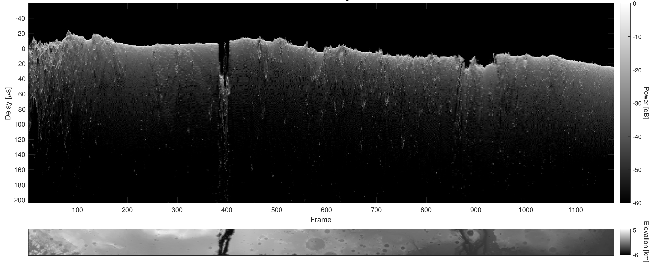
Orbit 16571, Cluttergram
