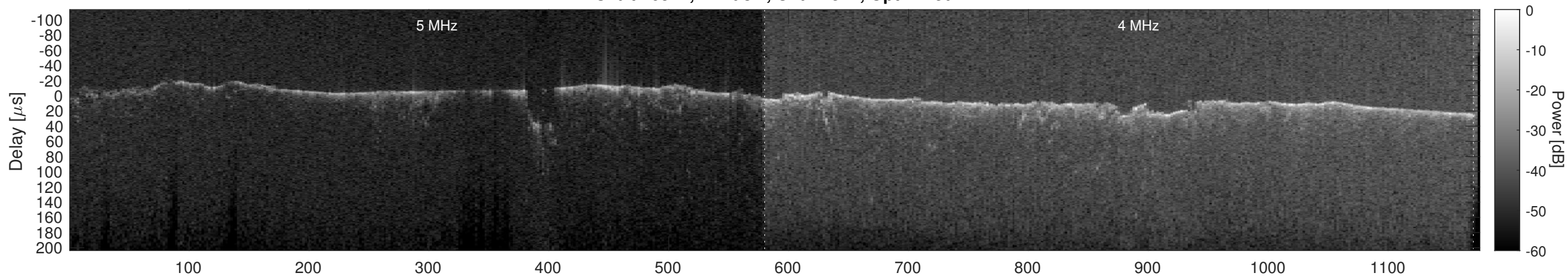
Orbit 16571, Cluttergram
