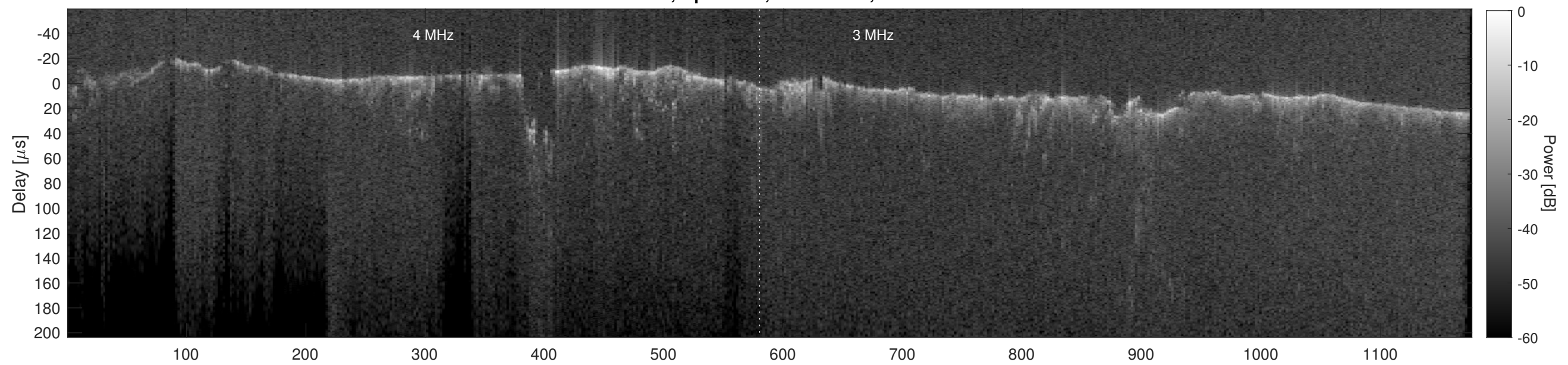
Orbit 16571, Cluttergram
