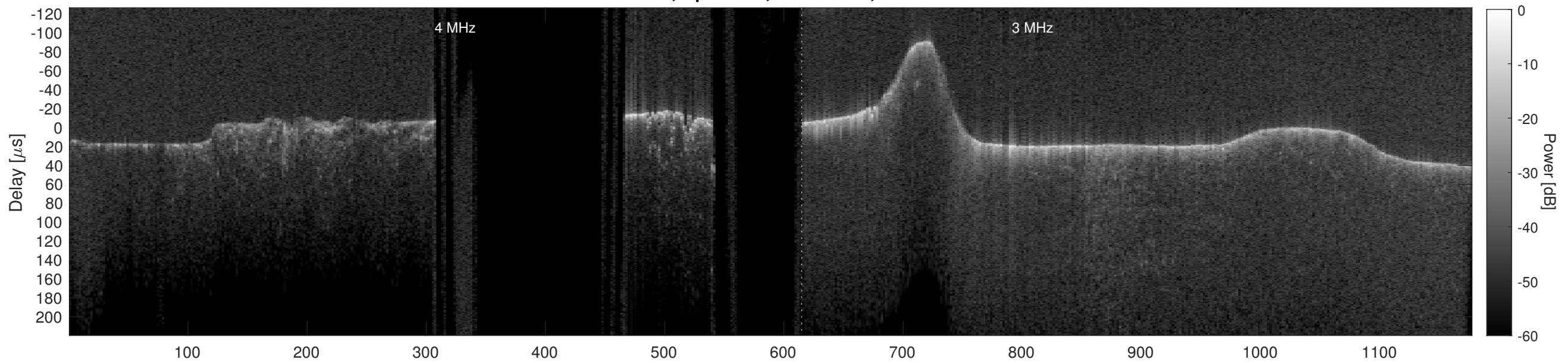
Orbit 16575, Cluttergram
