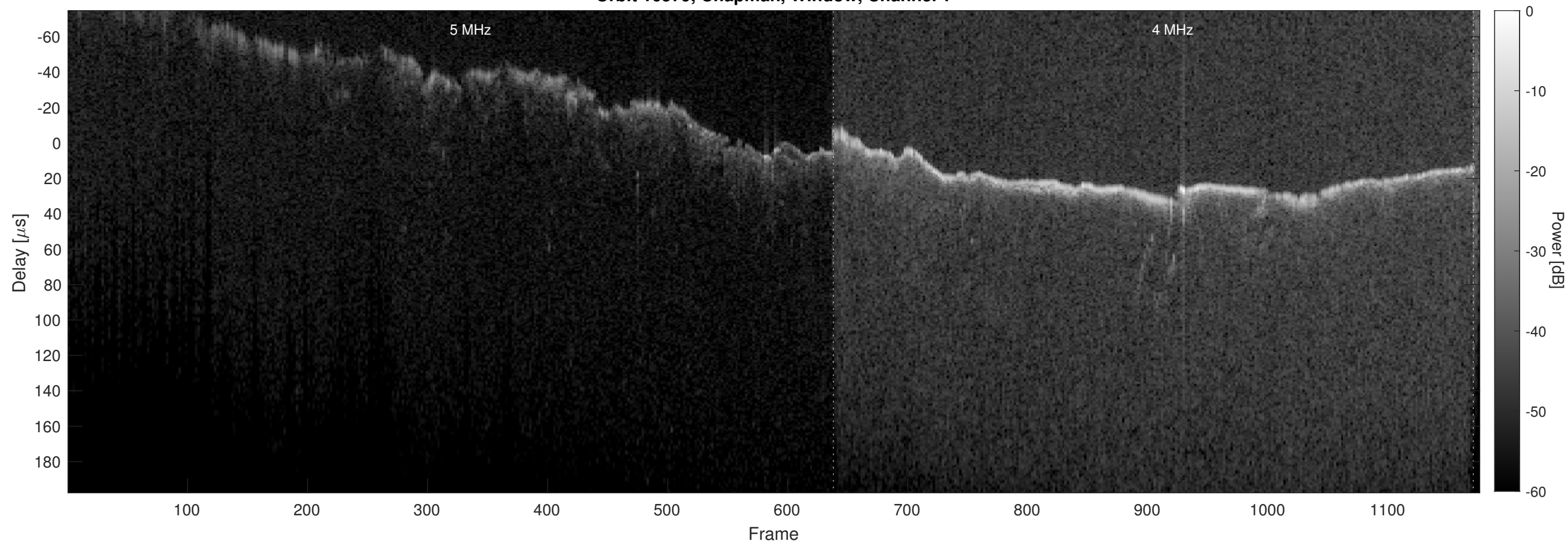
Orbit 16579, Chapman, Window, Channel 2
