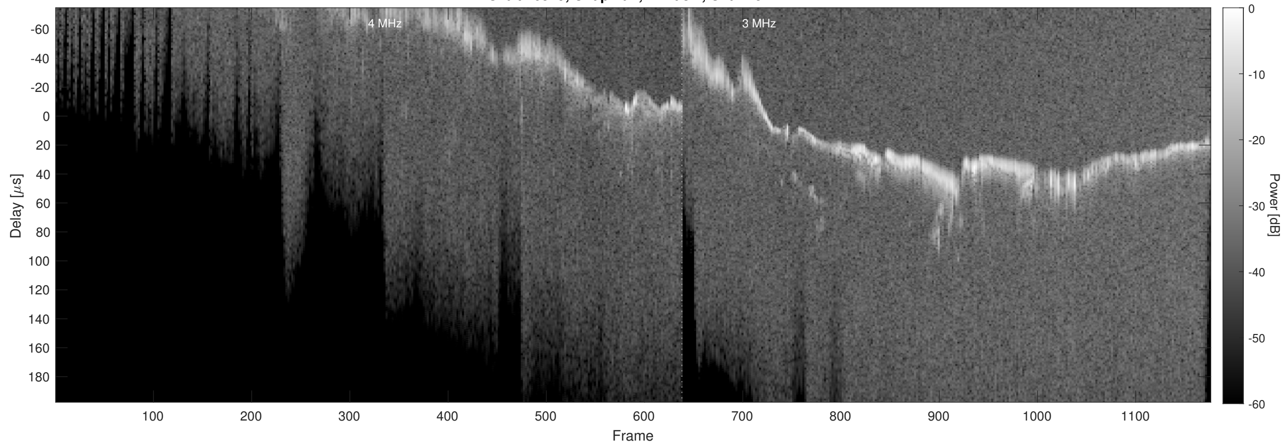
Orbit 16579, Chapman, Window, Channel 2
