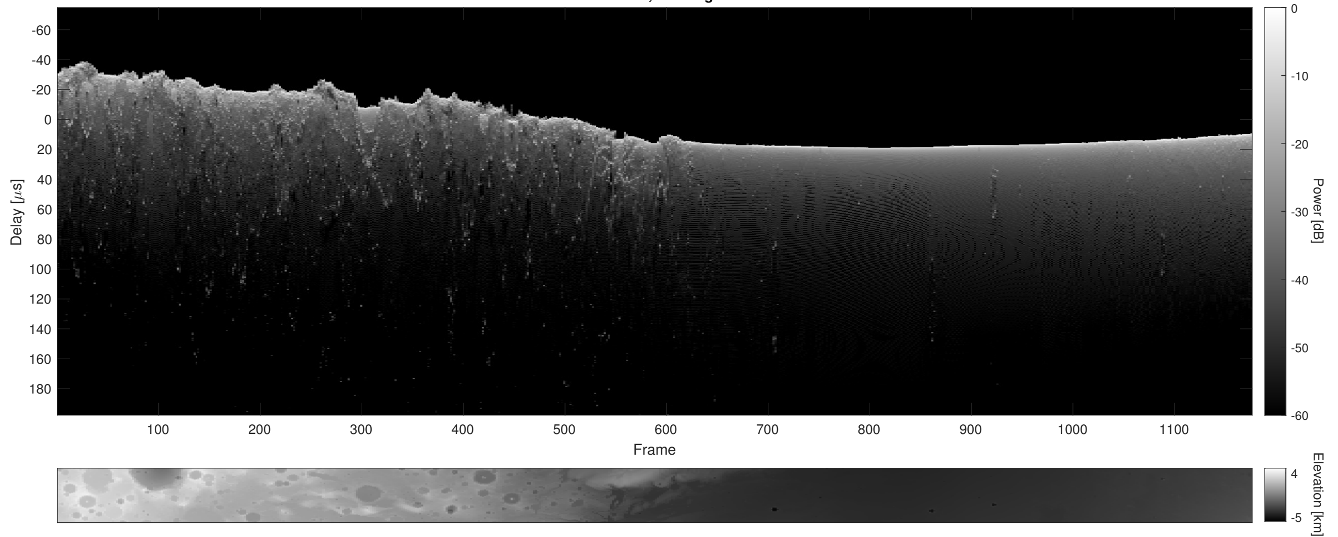
Orbit 16579, Cluttergram
