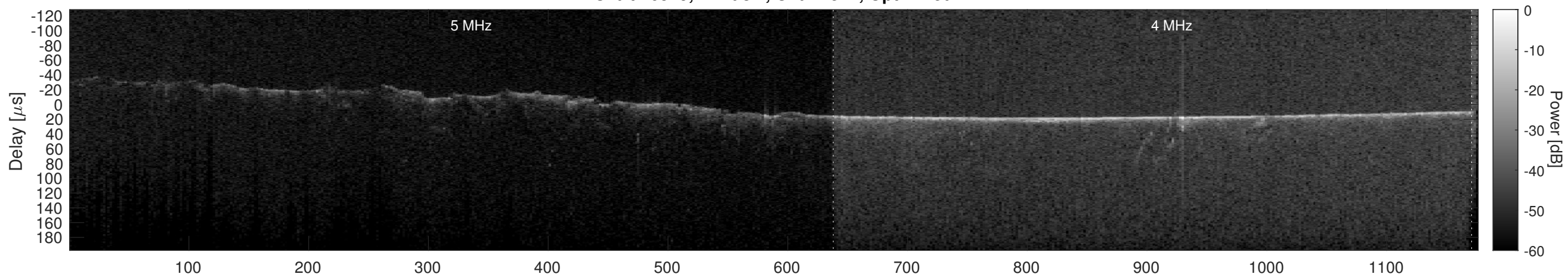
Orbit 16579, Cluttergram
