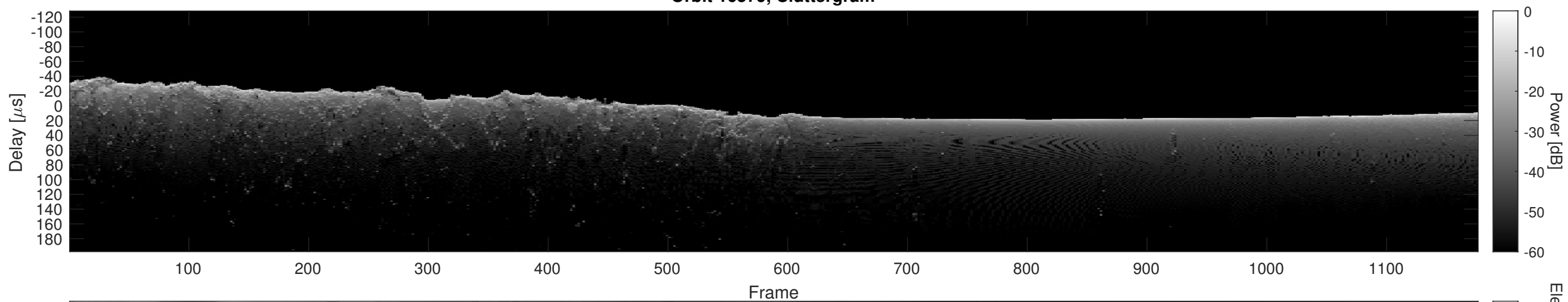
Orbit 16579, Cluttergram
