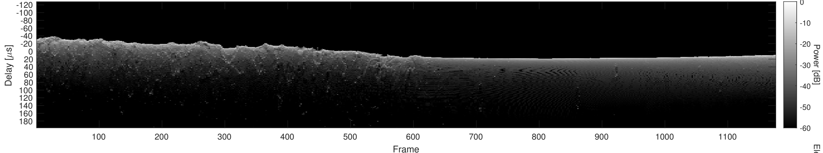
Orbit 16579, Cluttergram
