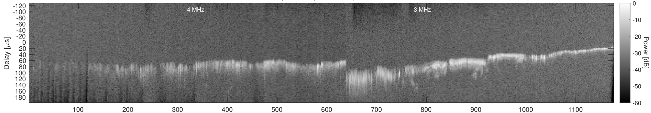
Orbit 16579, Window, Channel 2, Chapman
