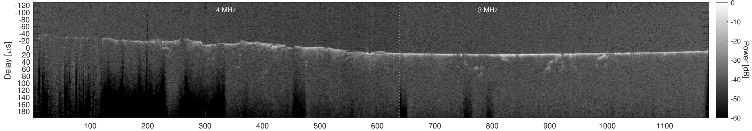
Orbit 16579, Cluttergram
