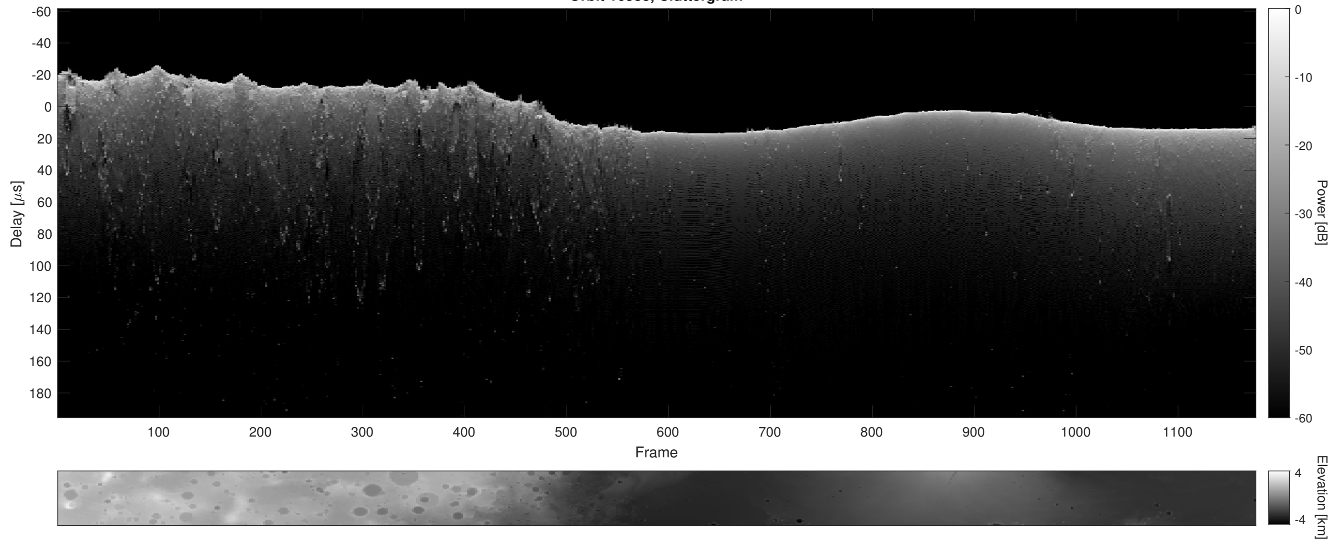
Orbit 16583, Cluttergram
