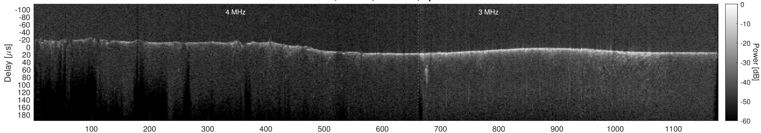
Orbit 16583, Cluttergram
