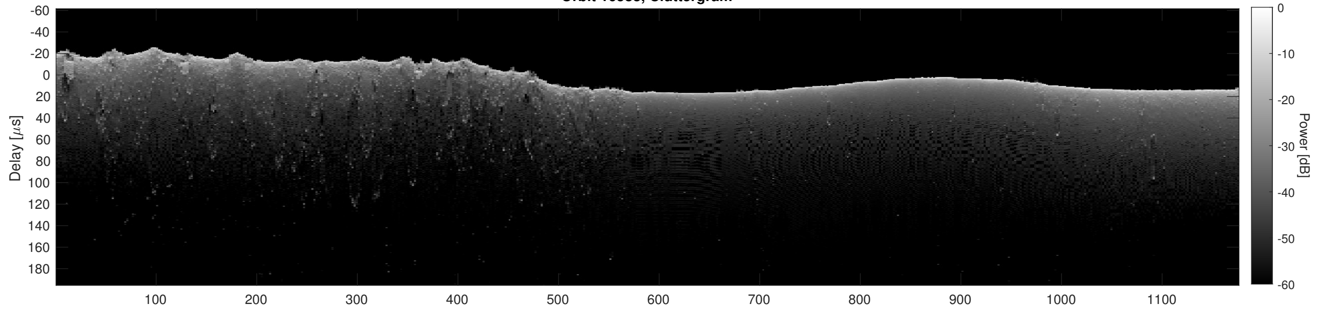
Orbit 16583, Cluttergram
