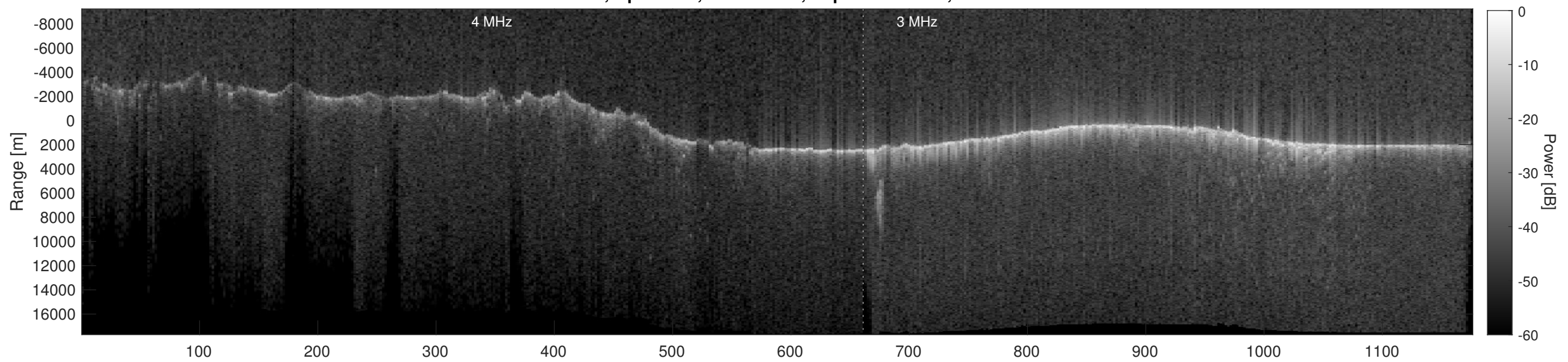
Orbit 16583, Depth-Corrected Cluttergram
