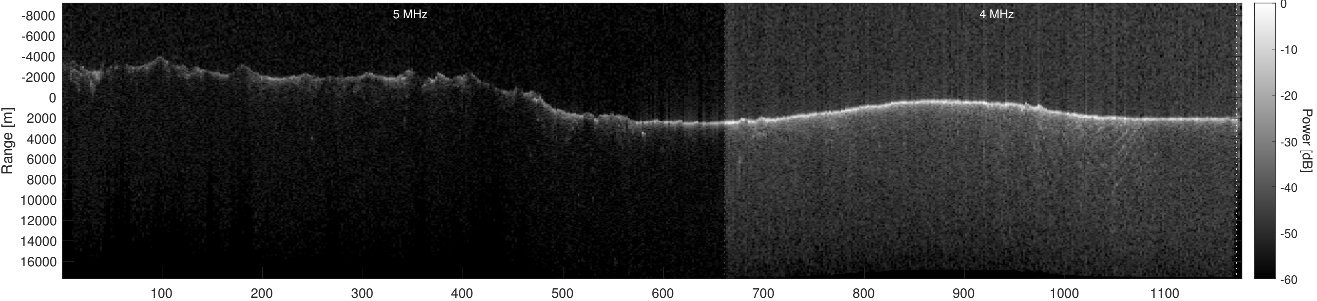
Orbit 16583, Optimized, Window, Depth-Corrected, Channel 2
