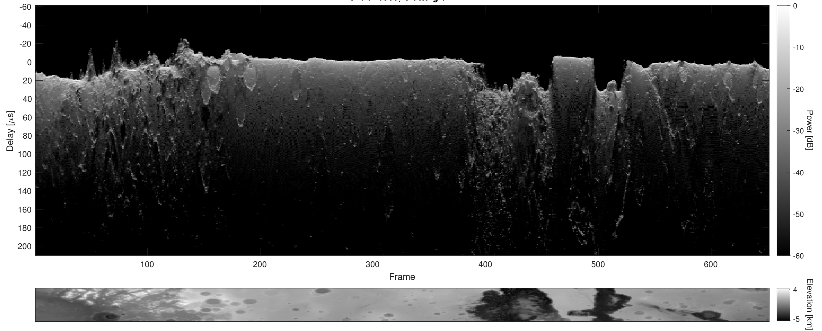
Orbit 16585, Cluttergram
