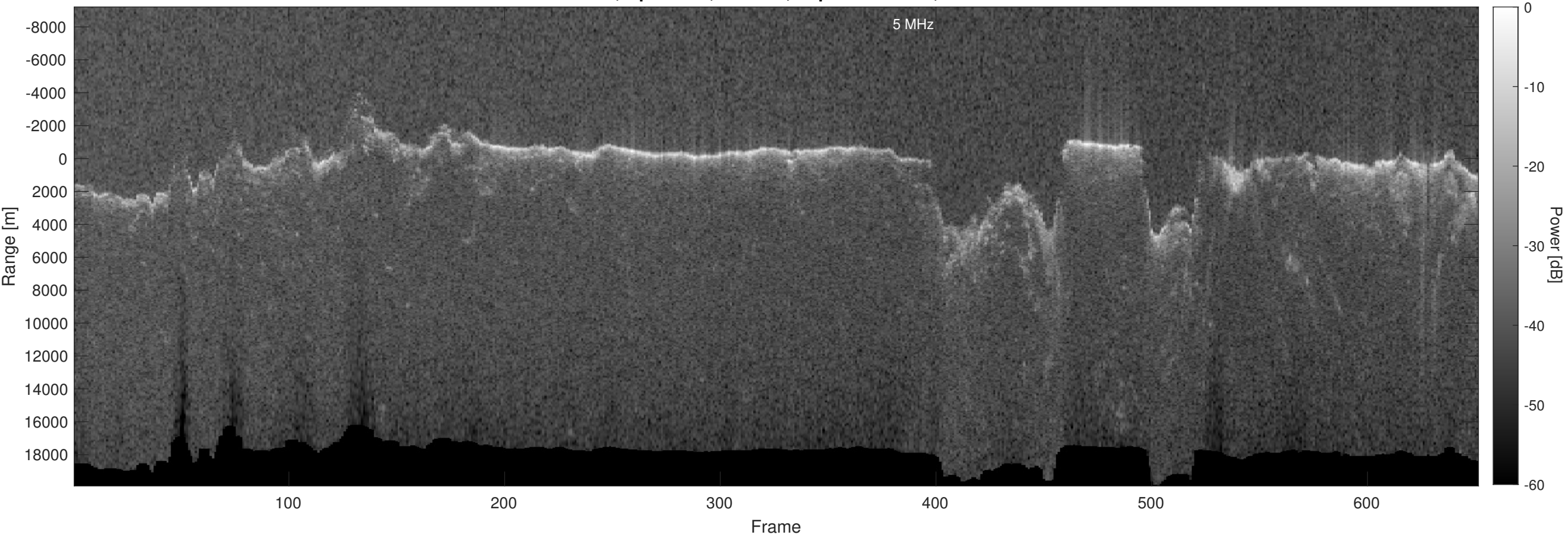
Orbit 16585, Optimized, Window, Depth-Corrected, Channel 2
