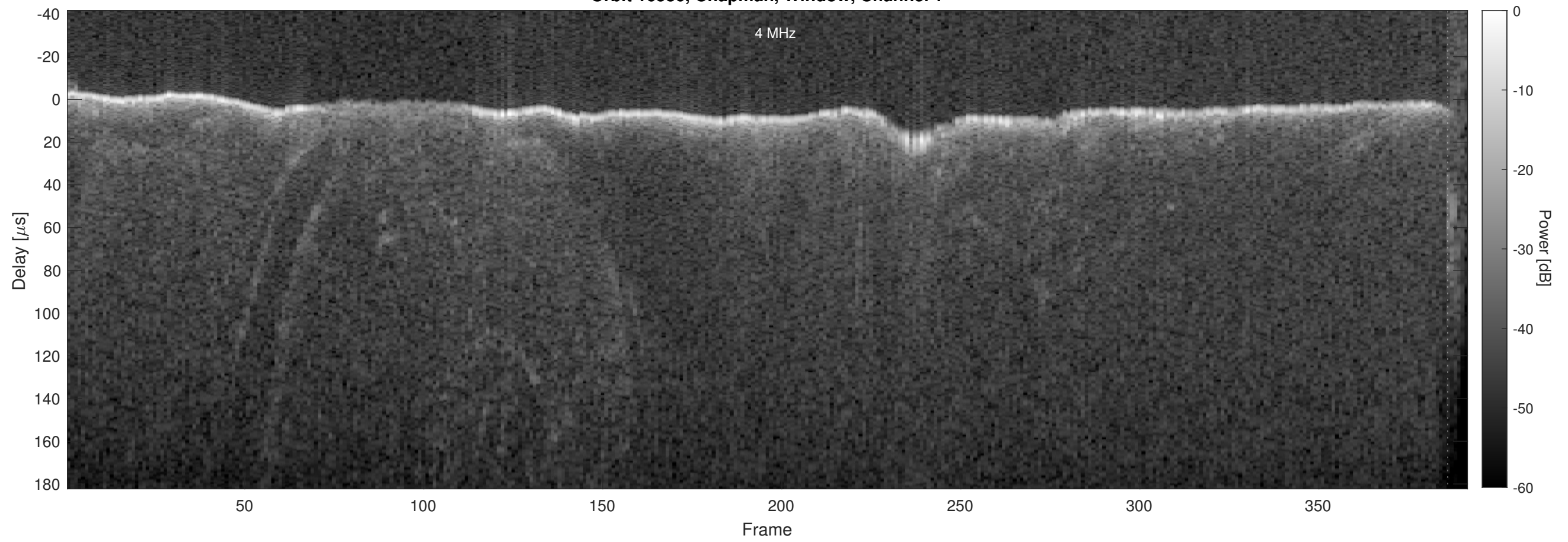
Orbit 16586, Chapman, Window, Channel 2
