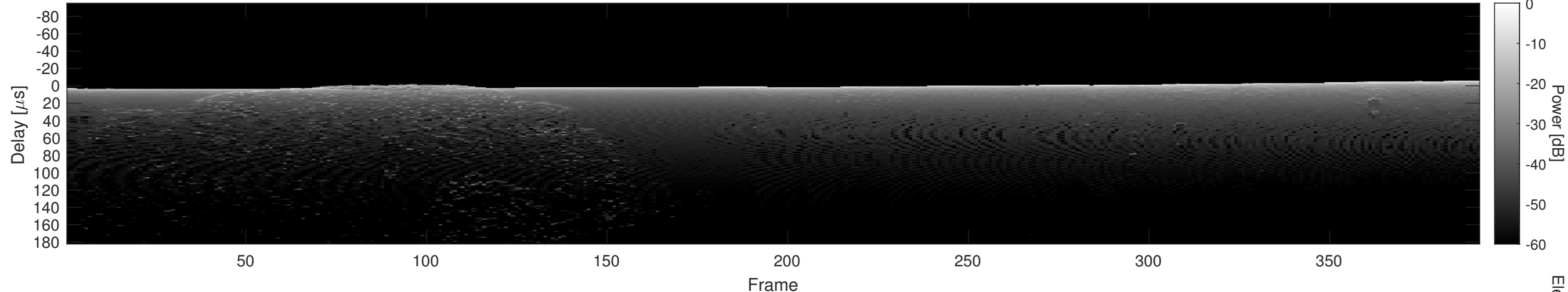
Orbit 16586, Cluttergram
