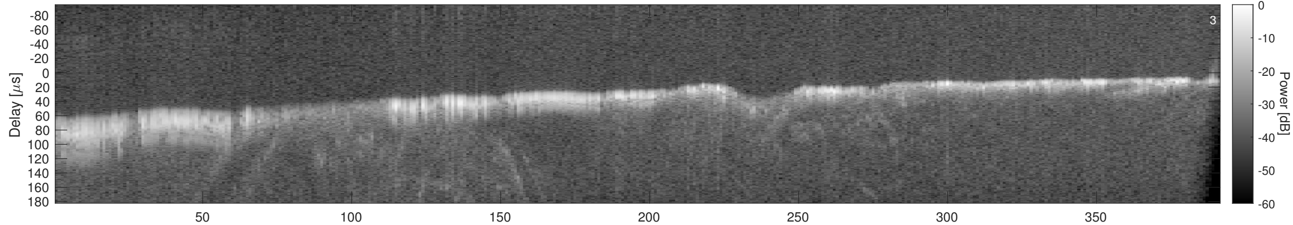
Orbit 16586, Window, Channel 2, Chapman
