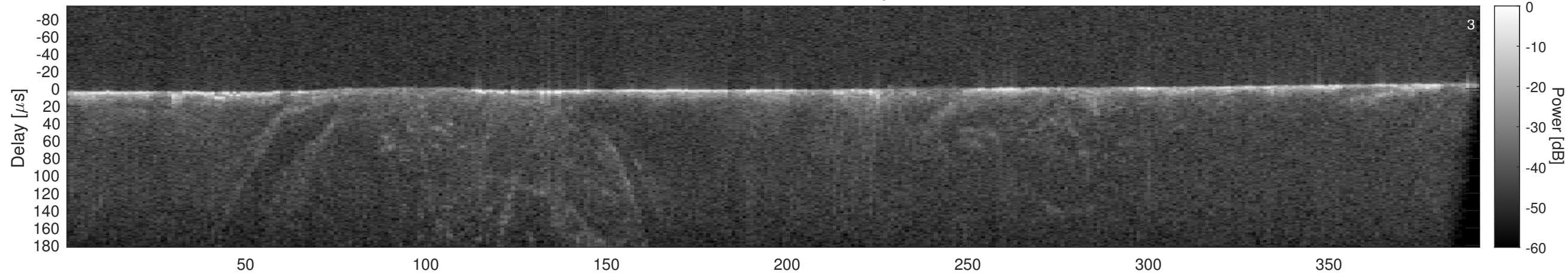
Orbit 16586, Cluttergram
