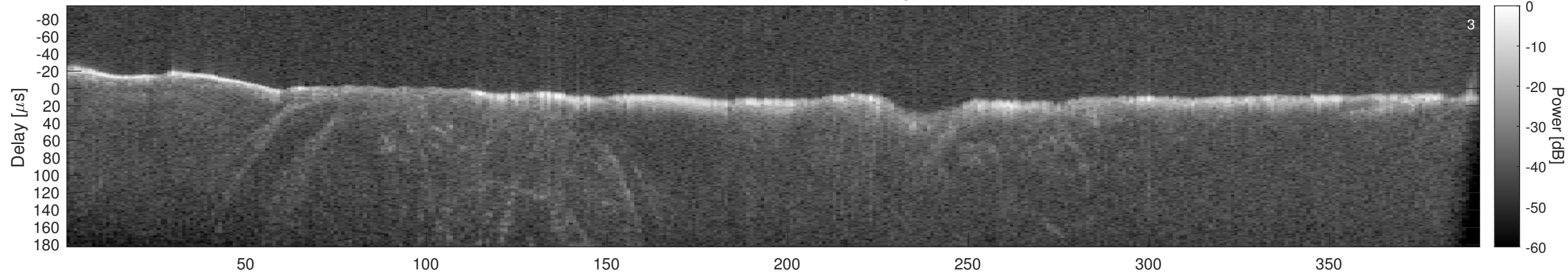
Orbit 16586, Window, Channel 2, Optimized
