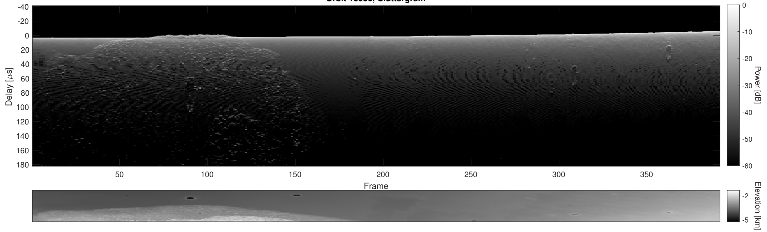
Orbit 16586, Cluttergram
