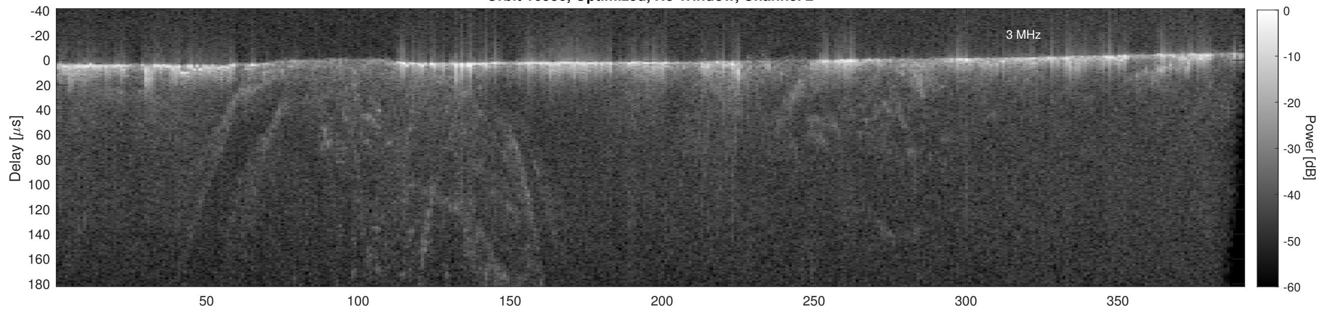
Orbit 16586, Cluttergram
