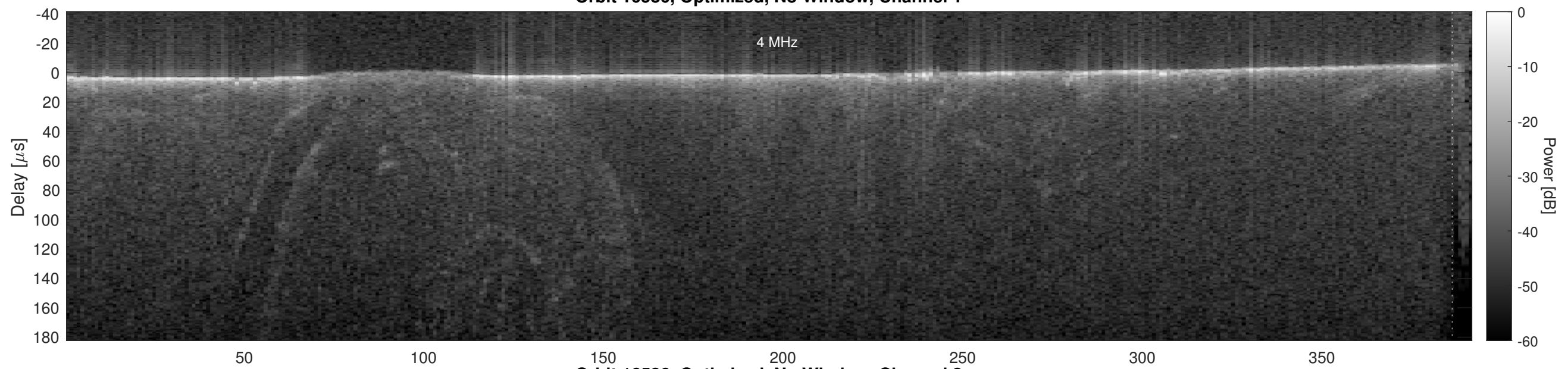
Orbit 16586, Optimized, No Window, Channel 2
