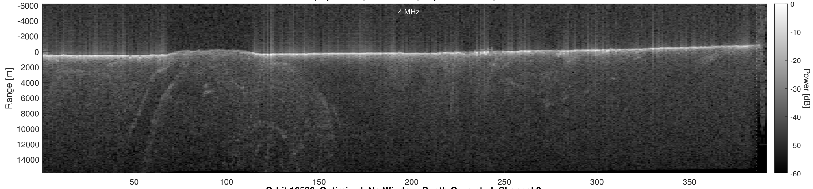
Orbit 16586, Optimized, No Window, Depth-Corrected, Channel 2
