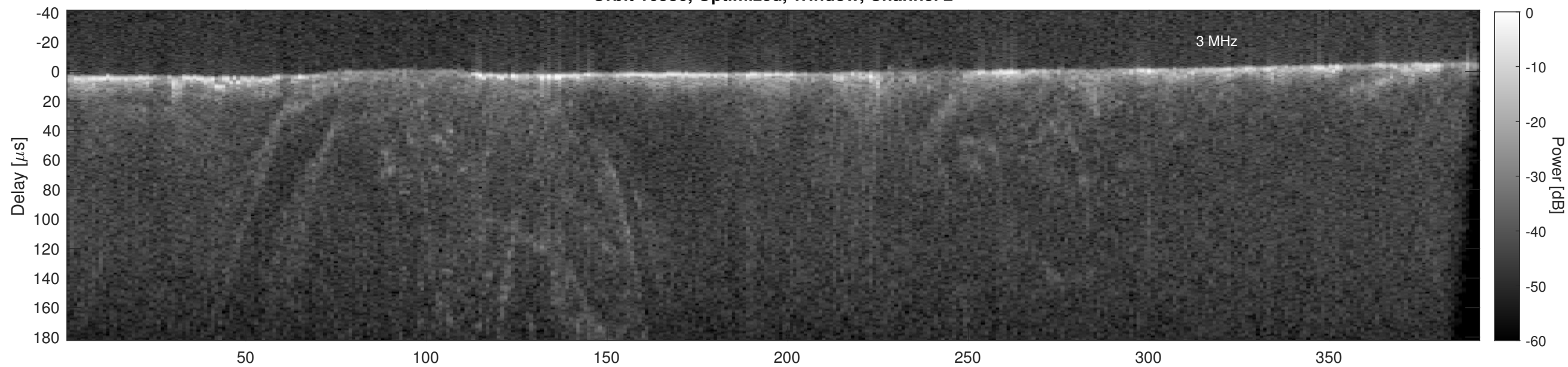
Orbit 16586, Cluttergram
