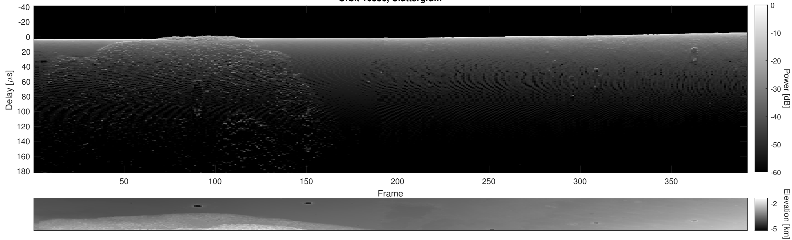
Orbit 16586, Cluttergram
