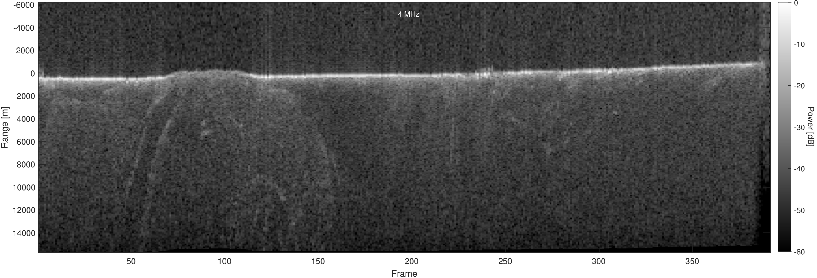
Orbit 16586, Optimized, Window, Depth-Corrected, Channel 2
