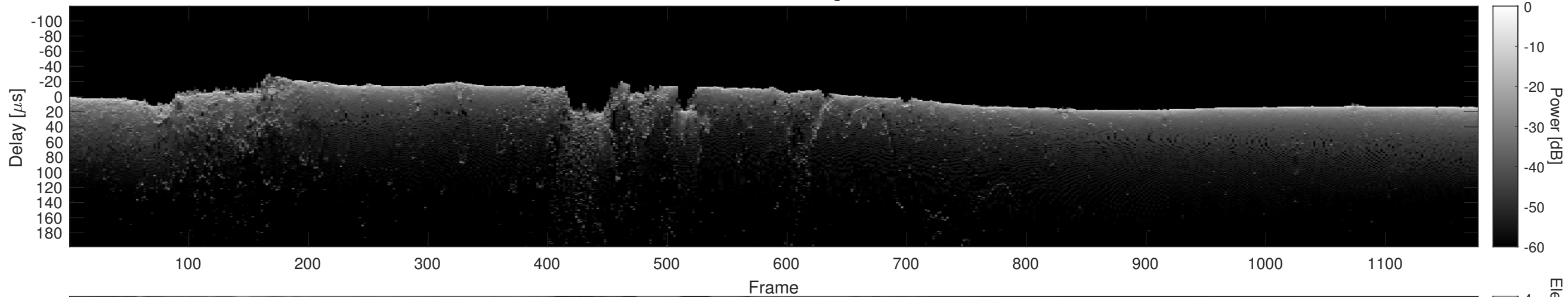
Orbit 16592, Cluttergram
