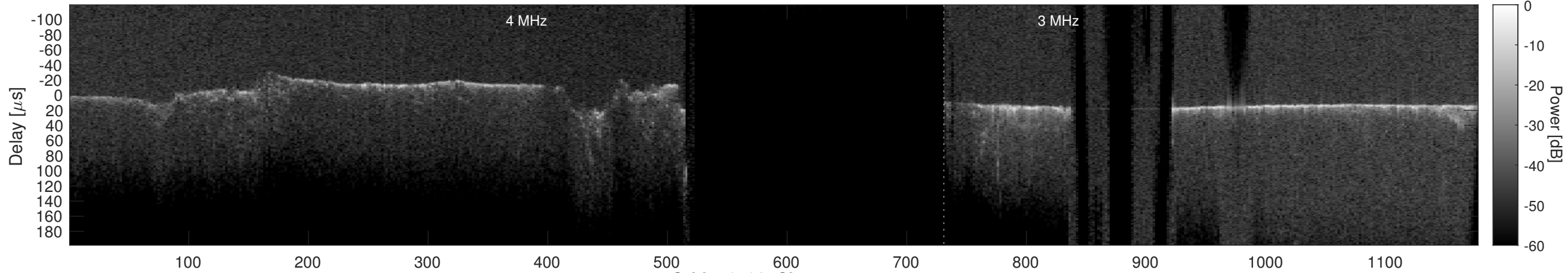
Orbit 16592, Cluttergram
