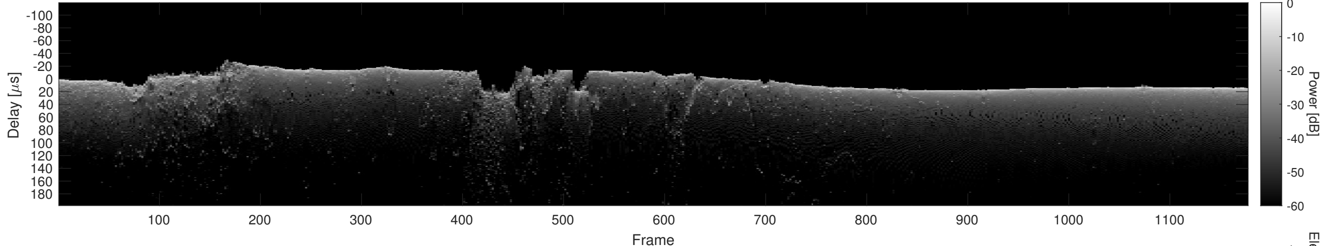
Orbit 16592, Cluttergram
