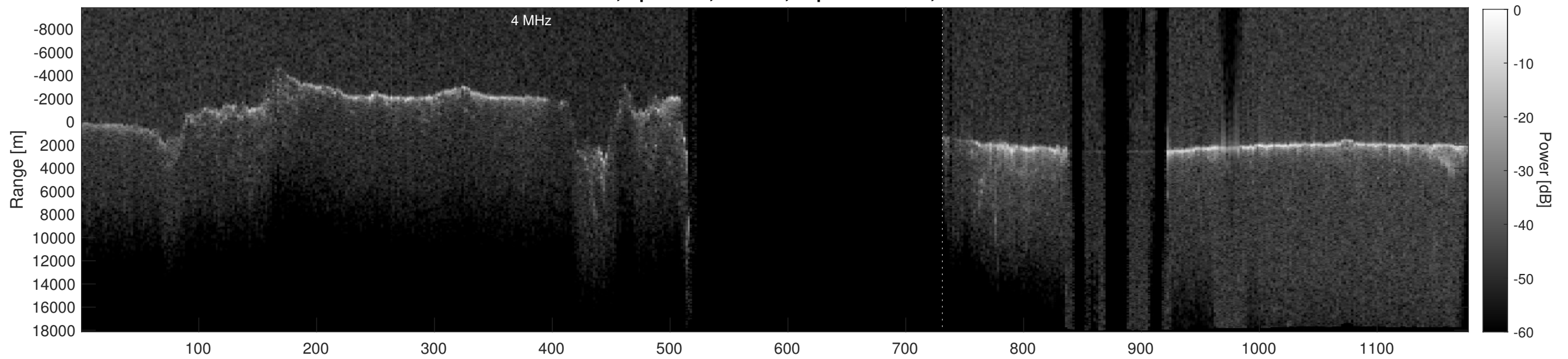
Orbit 16592, Depth-Corrected Cluttergram
