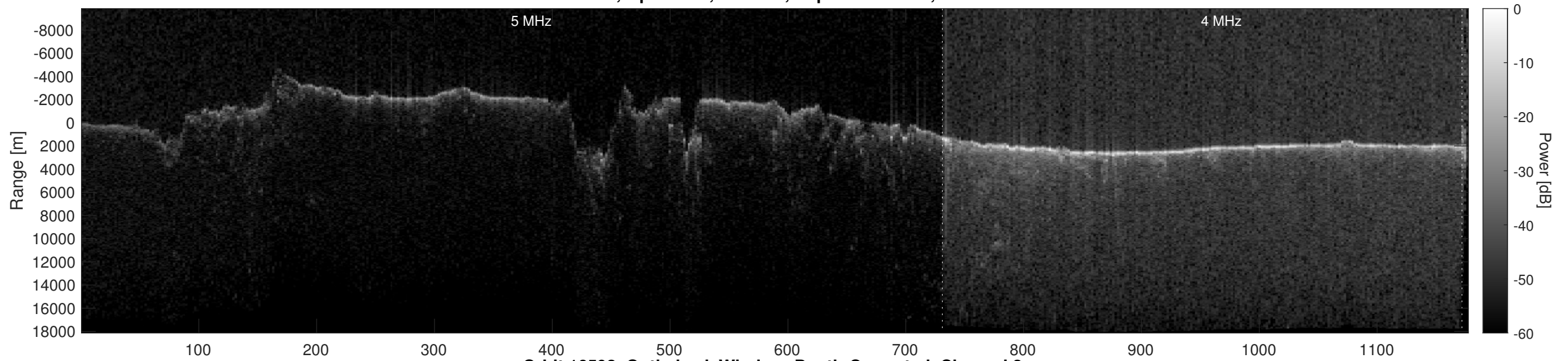
Orbit 16592, Optimized, Window, Depth-Corrected, Channel 2
