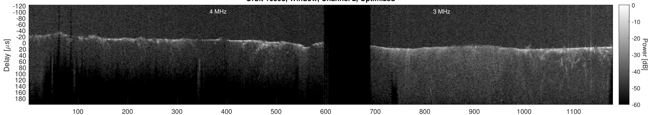
Orbit 16593, Cluttergram
