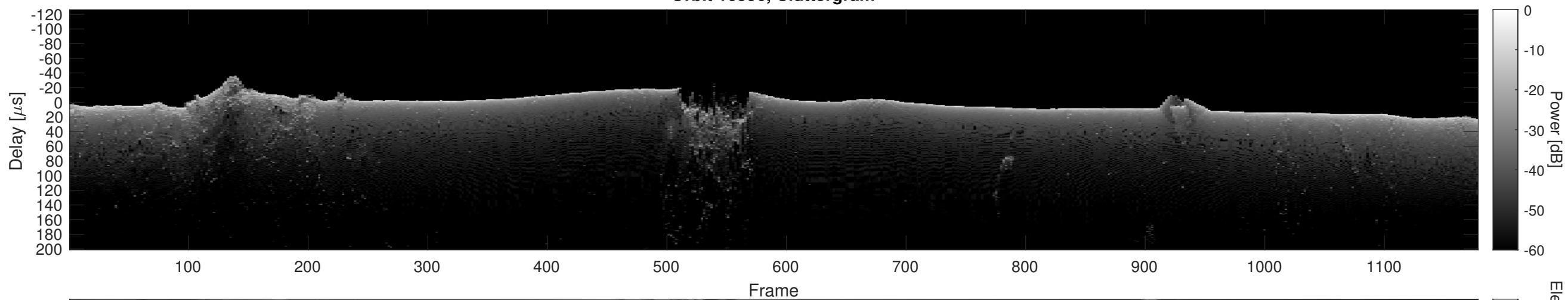
Orbit 16596, Cluttergram
