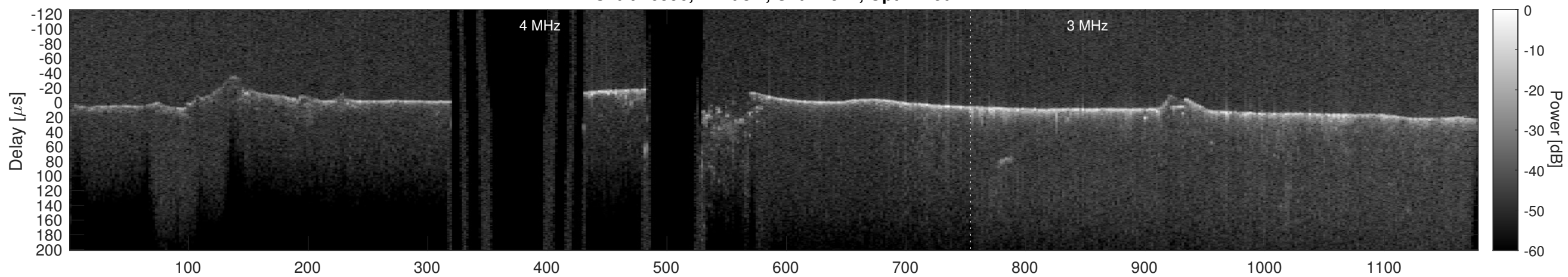
Orbit 16596, Cluttergram
