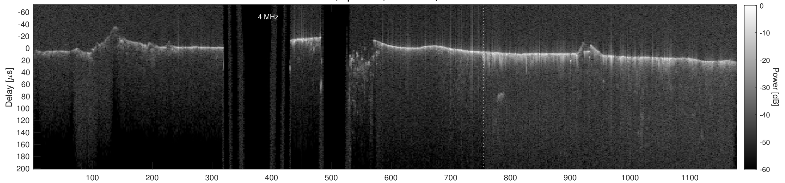
Orbit 16596, Cluttergram
