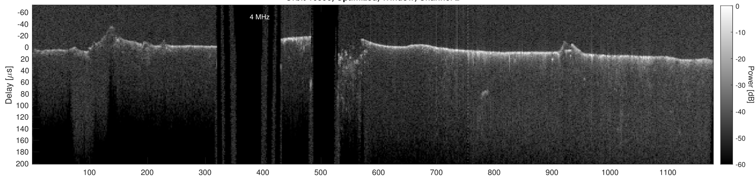
Orbit 16596, Cluttergram
