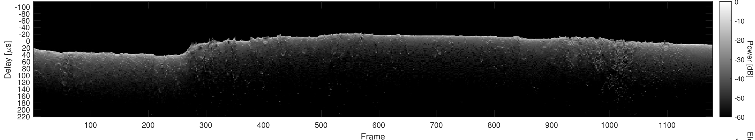
Orbit 16598, Cluttergram
