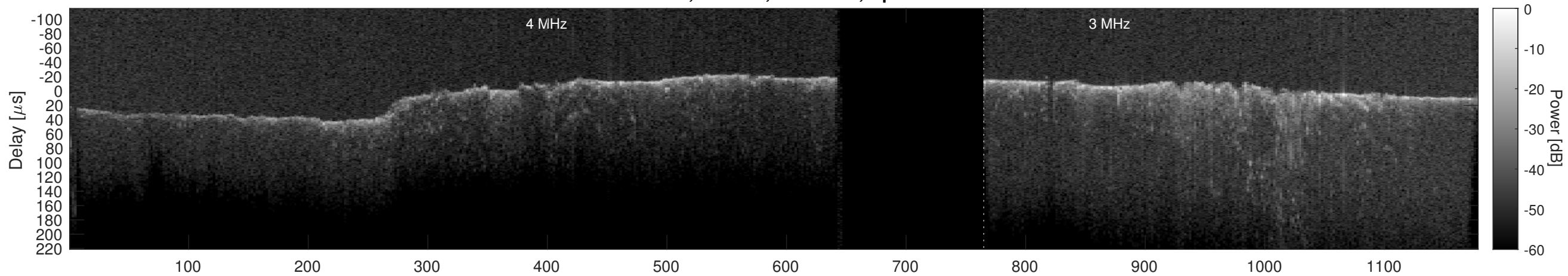
Orbit 16598, Cluttergram
