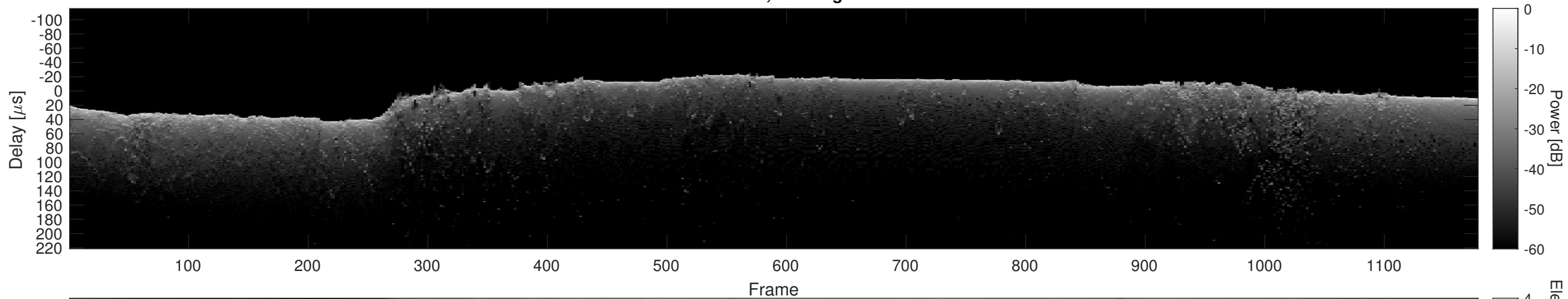
Orbit 16598, Cluttergram
