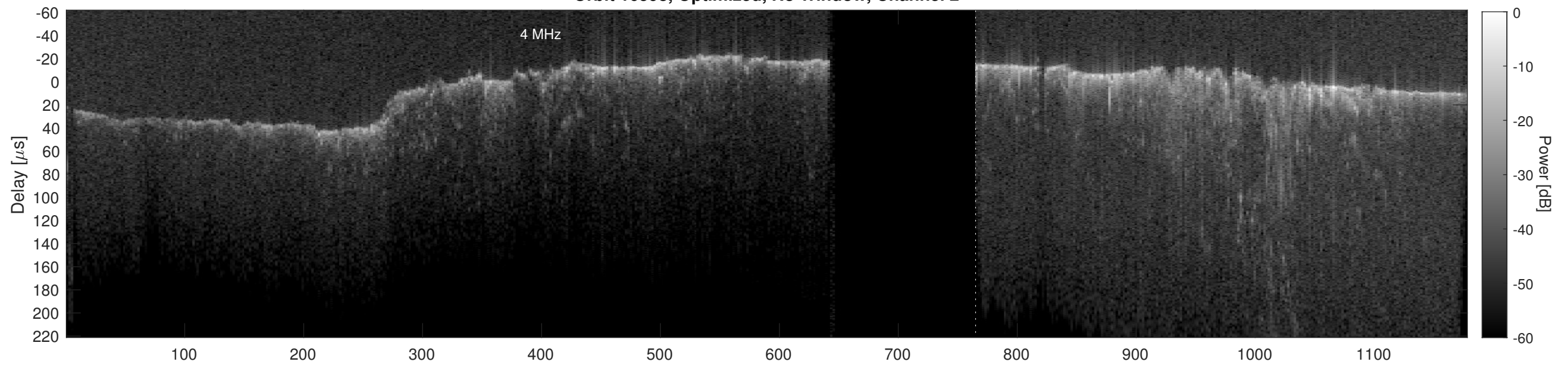
Orbit 16598, Cluttergram
