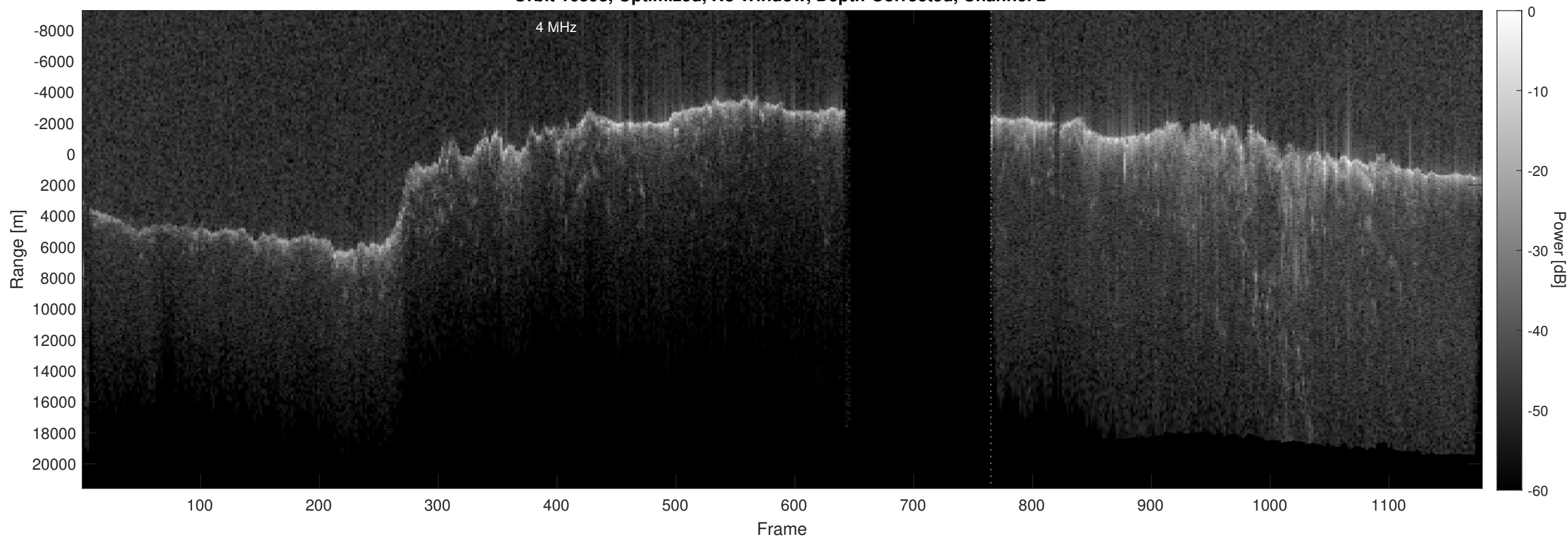
Orbit 16598, Optimized, No Window, Depth-Corrected, Channel 2
