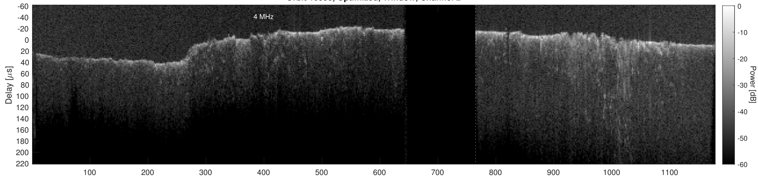
Orbit 16598, Cluttergram
