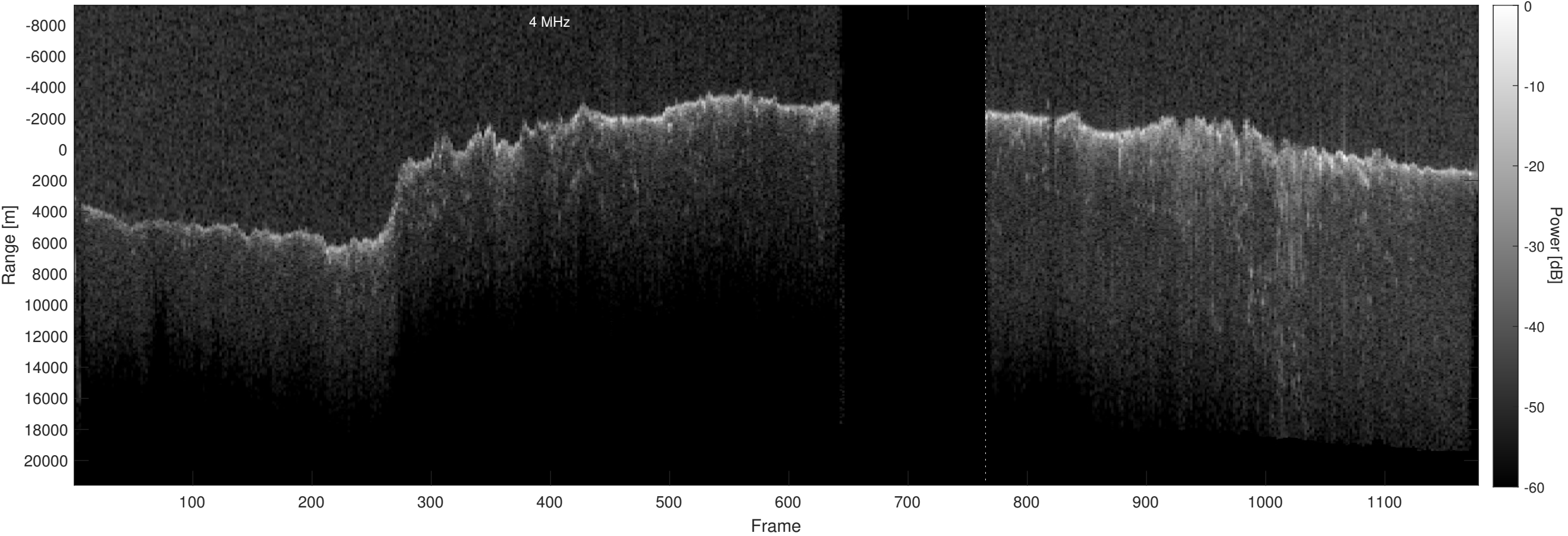
Orbit 16598, Optimized, Window, Depth-Corrected, Channel 2
