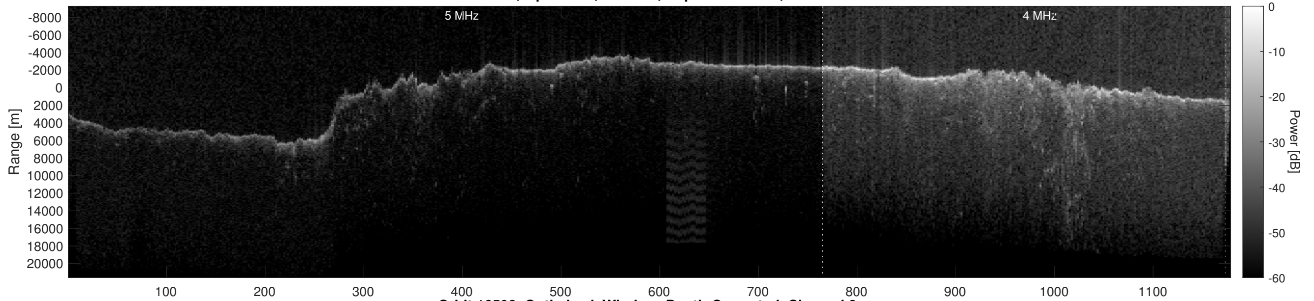
Orbit 16598, Optimized, Window, Depth-Corrected, Channel 2
