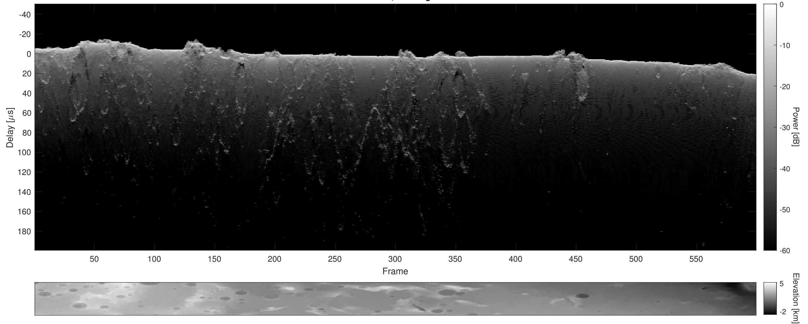
Orbit 16600, Cluttergram
