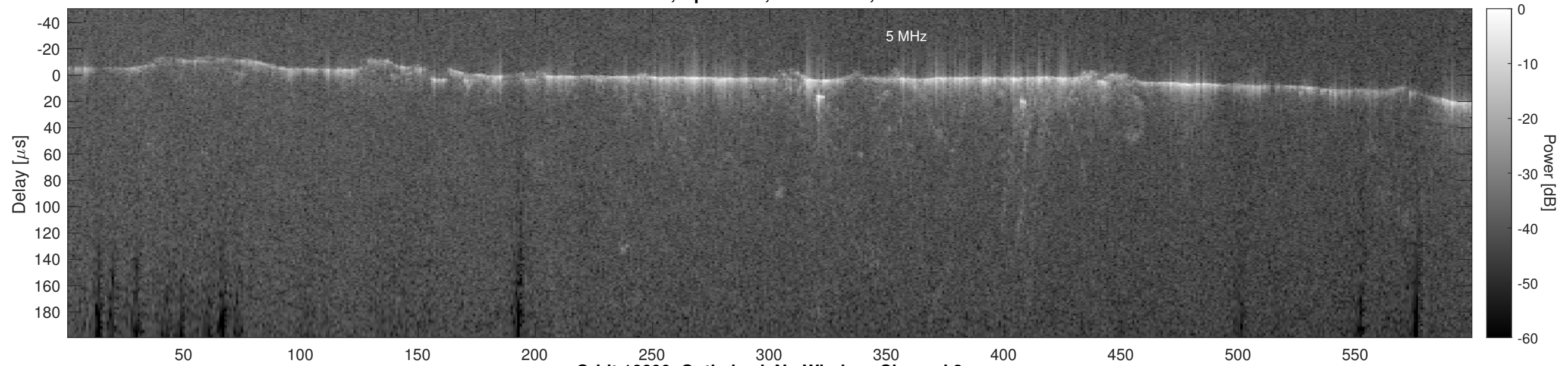
Orbit 16600, Optimized, No Window, Channel 2
