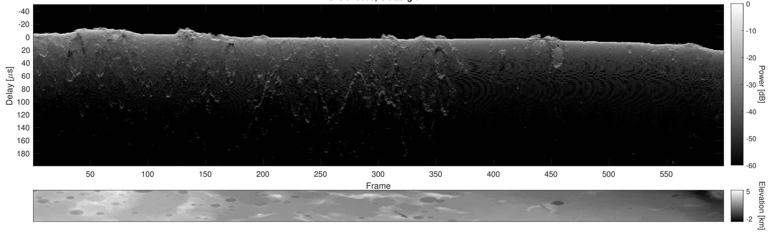
Orbit 16600, Cluttergram
