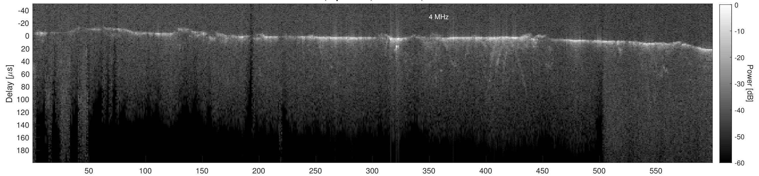
Orbit 16600, Cluttergram
