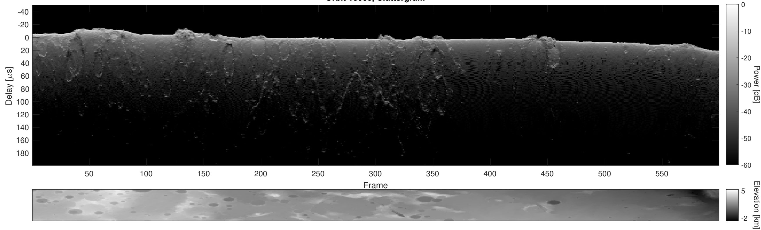
Orbit 16600, Cluttergram
