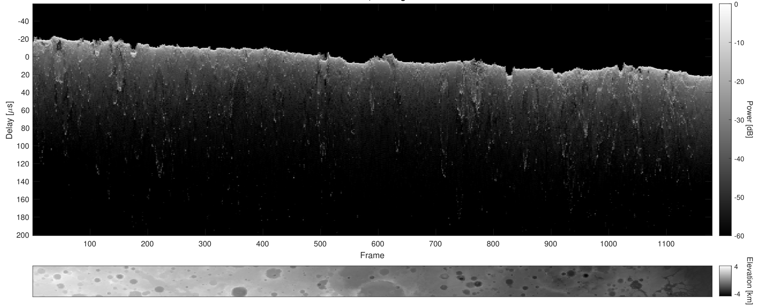
Orbit 16602, Cluttergram
