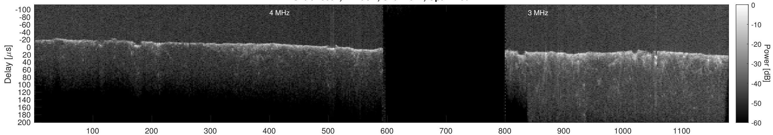
Orbit 16602, Cluttergram
