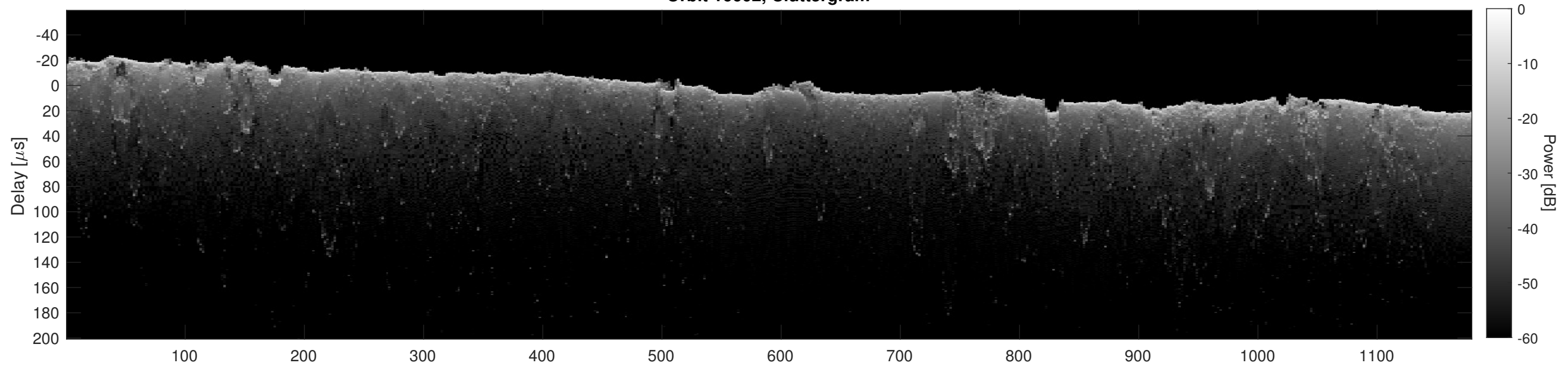
Orbit 16602, Cluttergram
