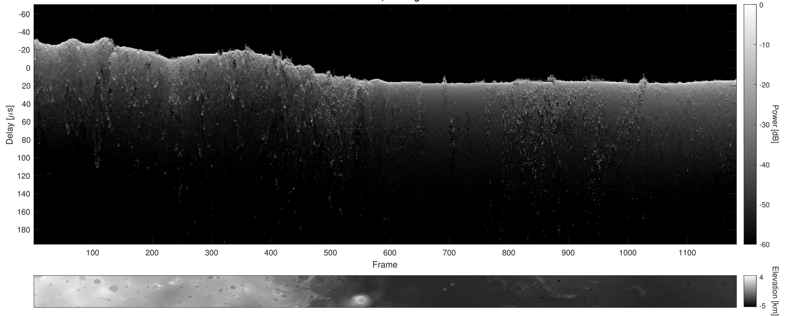
Orbit 16611, Cluttergram
